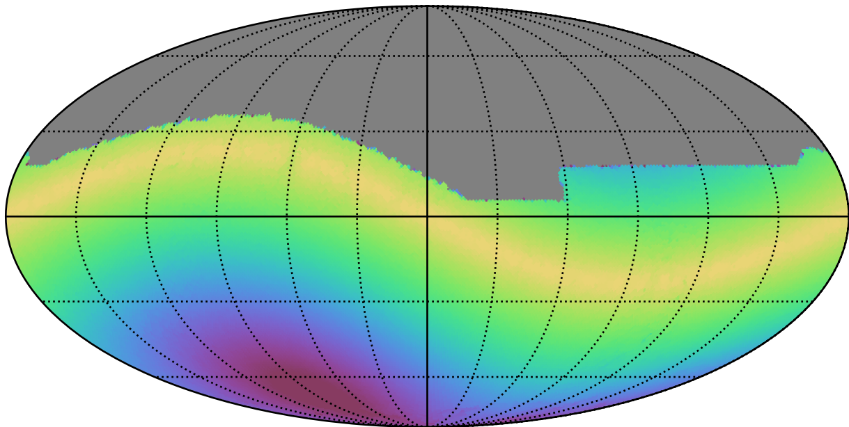
noroll_mjdp120_v3.4_10yrs All sky r band: Max solarElong
