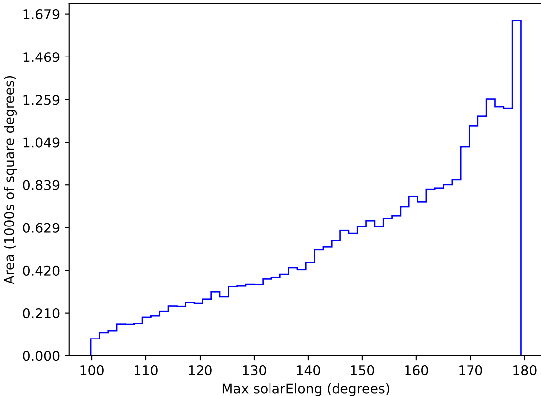
noroll_mjdp120_v3.4_10yrs All sky i band: Max solarElong
