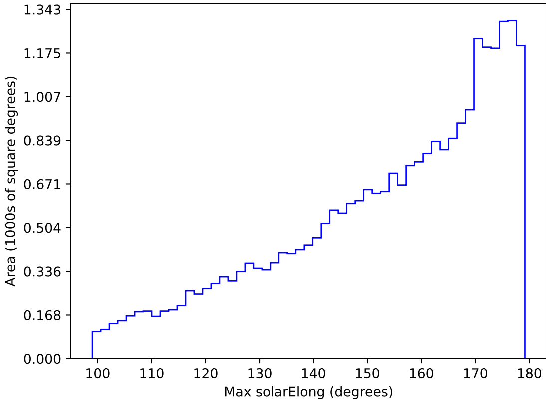
noroll_mjdp120_v3.4_10yrs All sky g band: Max solarElong
