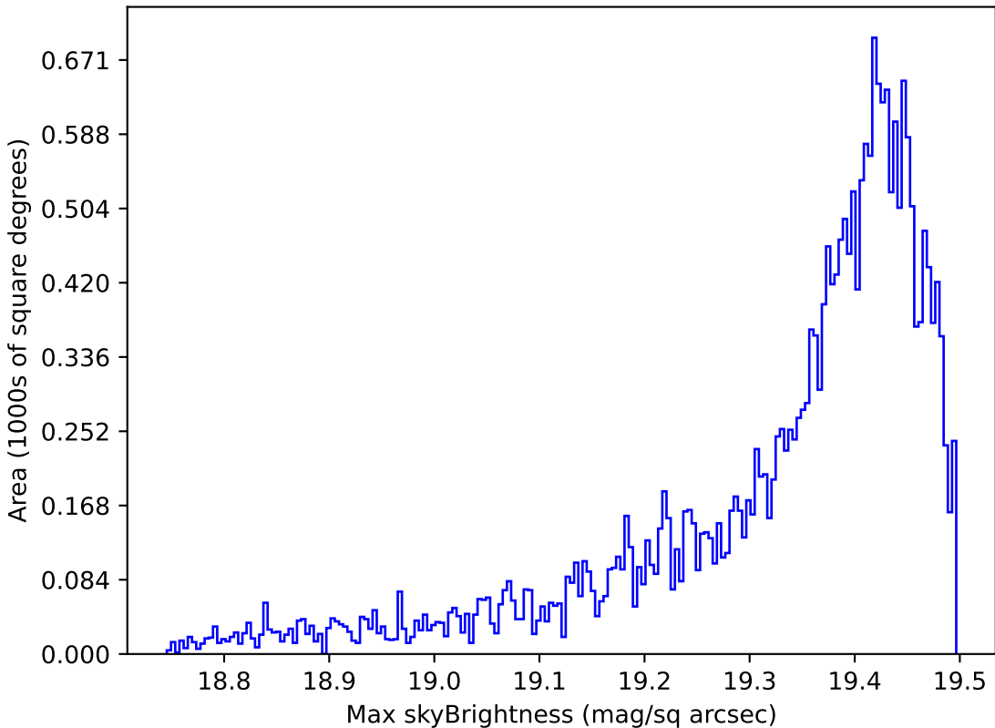
noroll_mjdp120_v3.4_10yrs Yr 1 z band: Max skyBrightness
