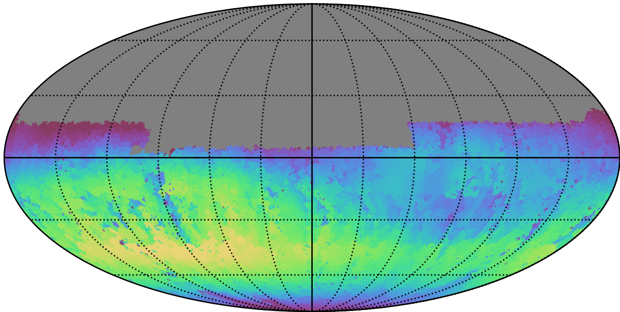
noroll_mjdp120_v3.4_10yrs Yr 1 u band: Max skyBrightness
