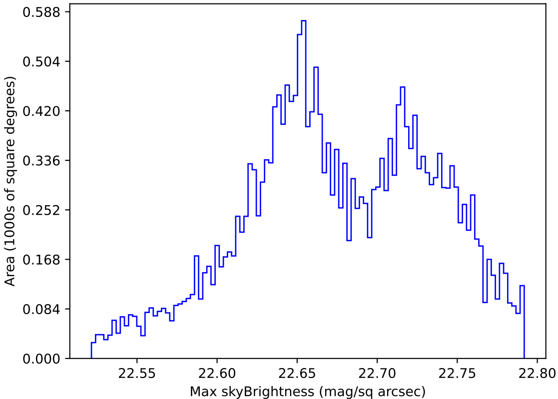
noroll_mjdp120_v3.4_10yrs Yr 1 u band: Max skyBrightness
