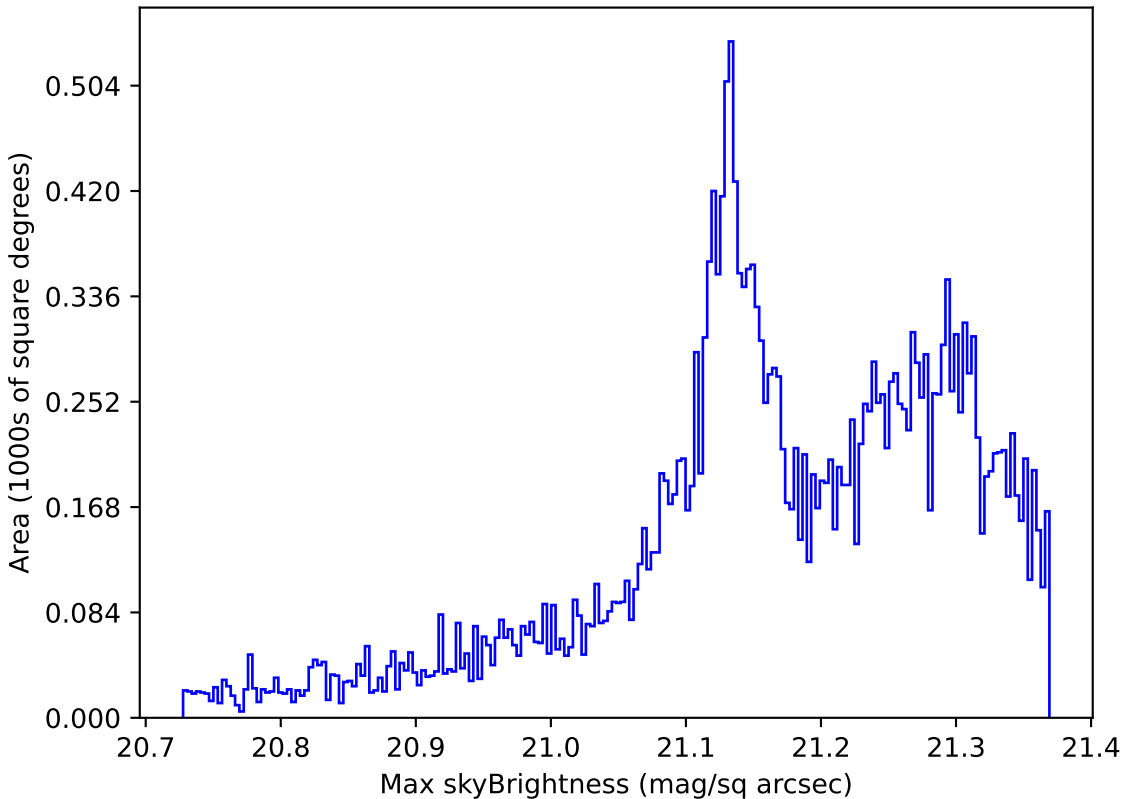
noroll_mjdp120_v3.4_10yrs Yr 1 r band: Max skyBrightness
