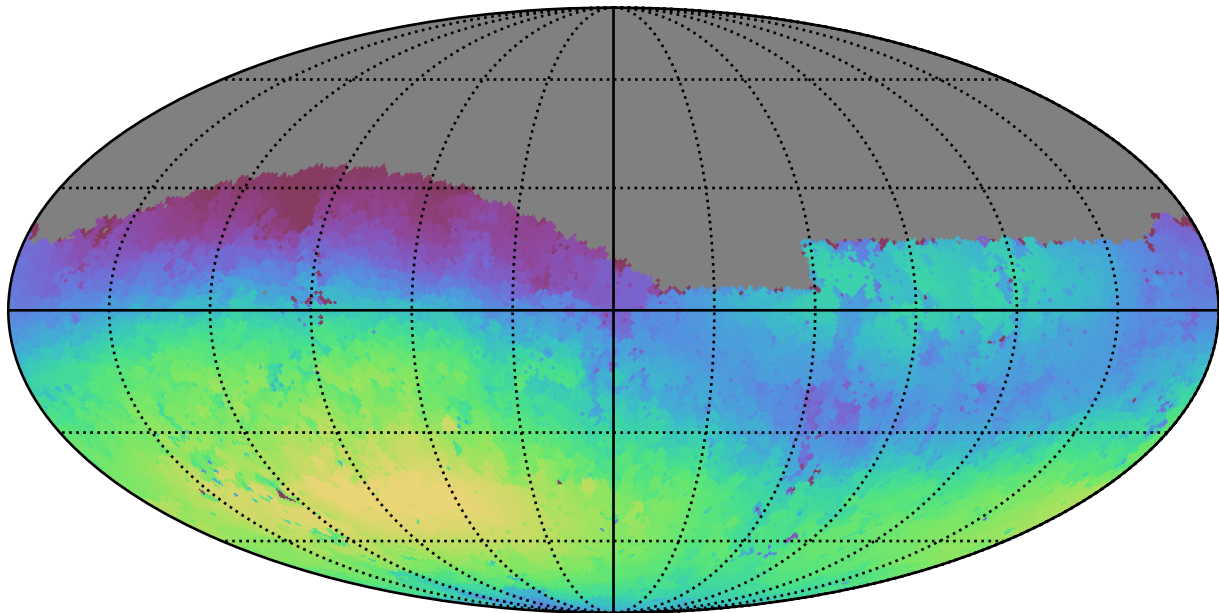
noroll_mjdp120_v3.4_10yrs Yr 1 g band: Max skyBrightness
