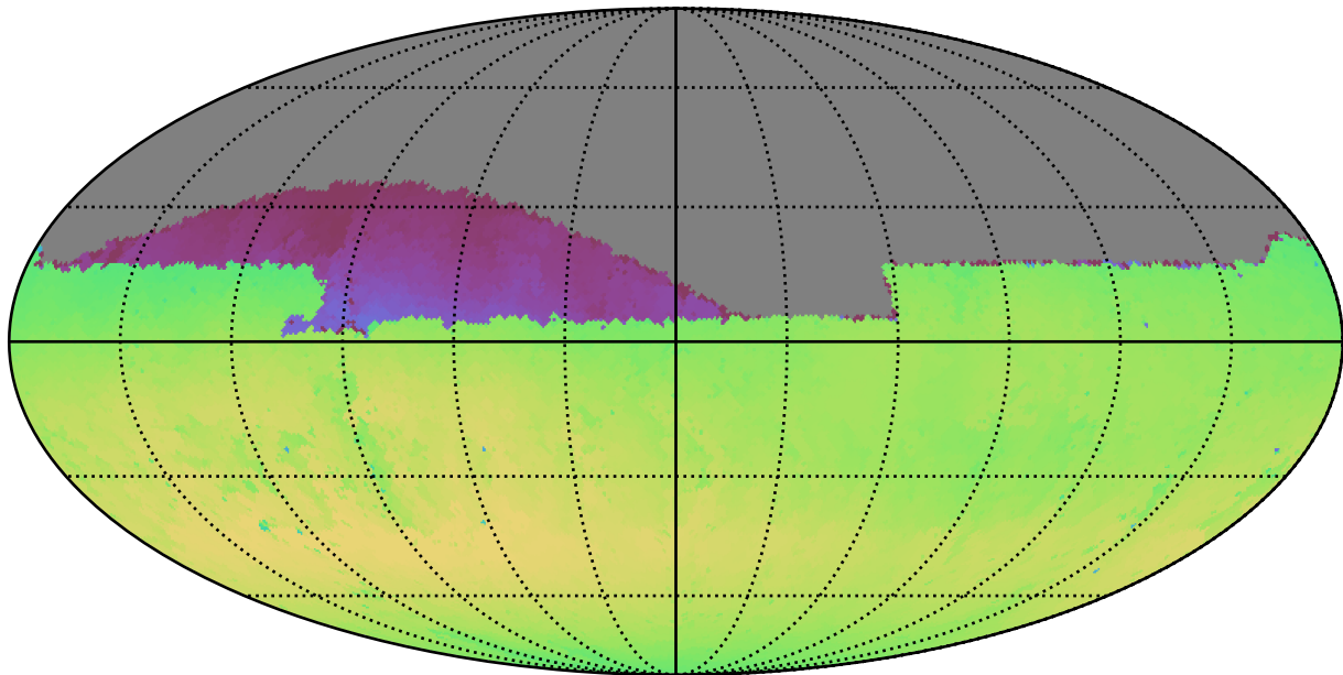
noroll_mjdp120_v3.4_10yrs Yr 1 all bands: Max skyBrightness
