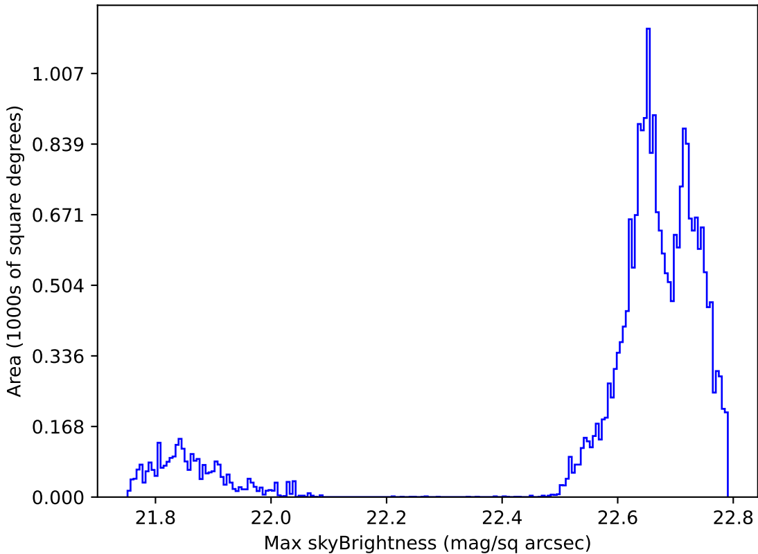
noroll_mjdp120_v3.4_10yrs Yr 1 all bands: Max skyBrightness
