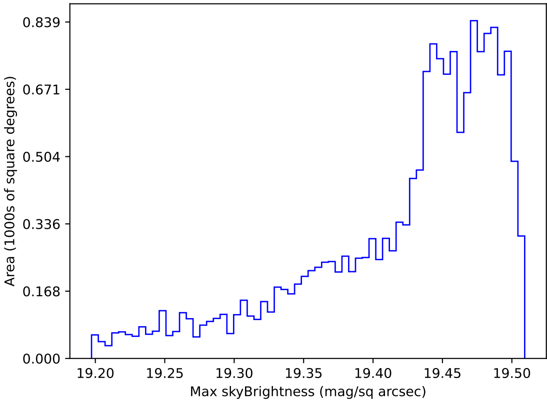
noroll_mjdp120_v3.4_10yrs WFD z band: Max skyBrightness
