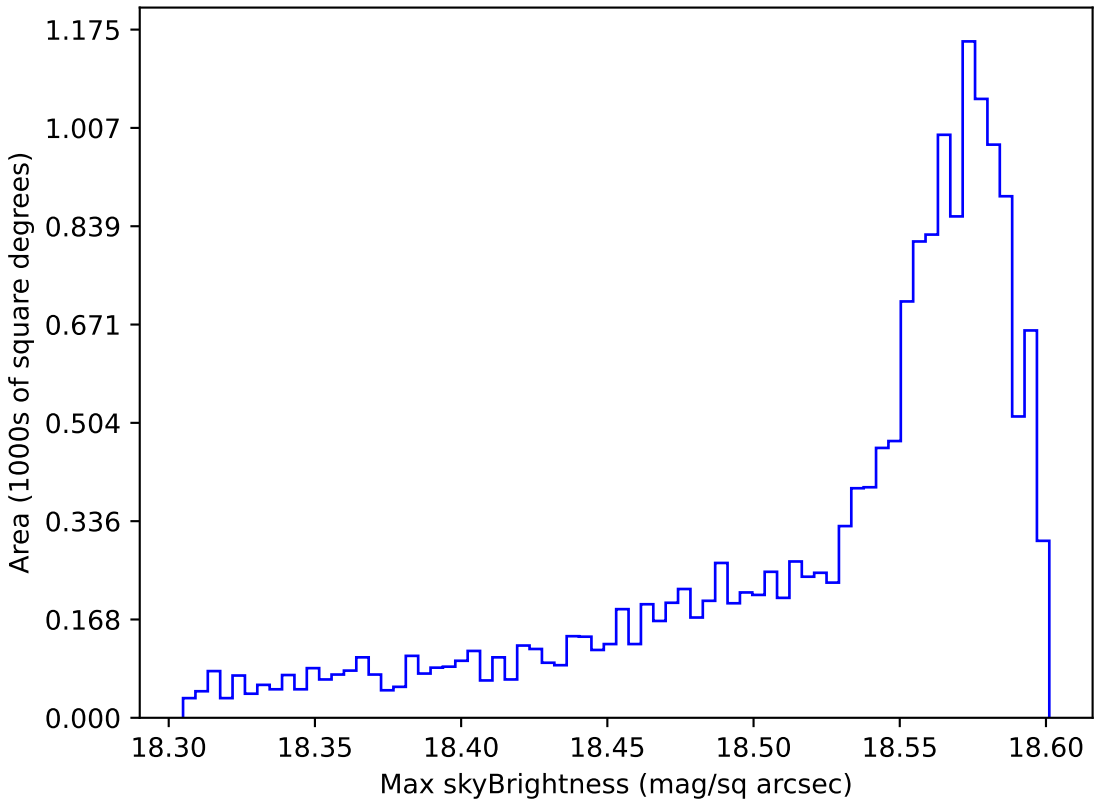
noroll_mjdp120_v3.4_10yrs WFD y band: Max skyBrightness
