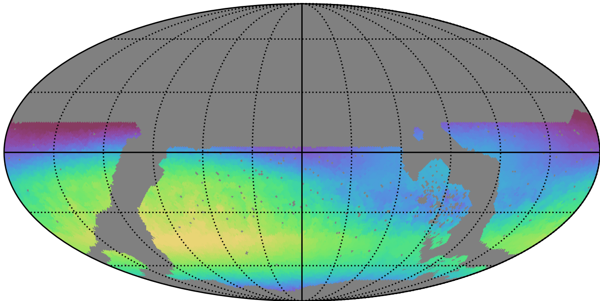
noroll_mjdp120_v3.4_10yrs WFD u band: Max skyBrightness
