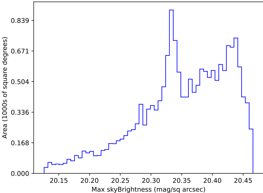
noroll_mjdp120_v3.4_10yrs WFD i band: Max skyBrightness
