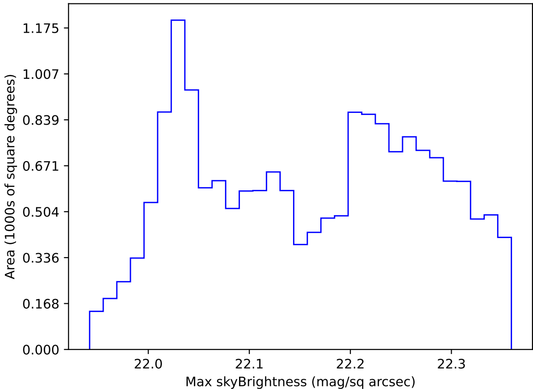
noroll_mjdp120_v3.4_10yrs WFD g band: Max skyBrightness
