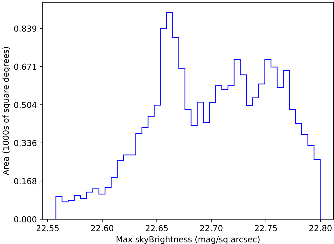
noroll_mjdp120_v3.4_10yrs WFD all bands: Max skyBrightness
