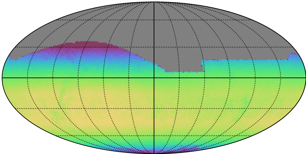
noroll_mjdp120_v3.4_10yrs All sky z band: Max skyBrightness
