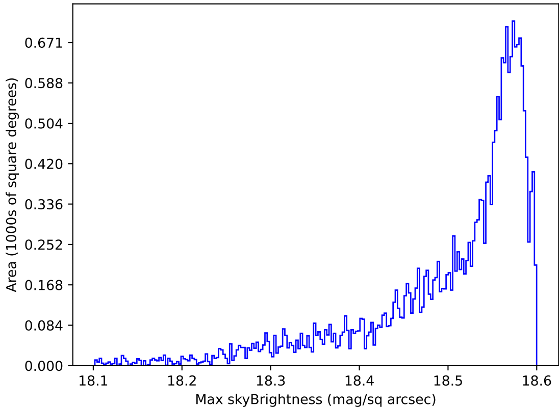
noroll_mjdp120_v3.4_10yrs All sky y band: Max skyBrightness
