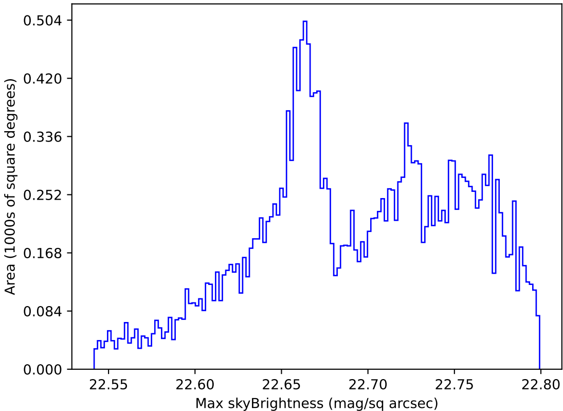
noroll_mjdp120_v3.4_10yrs All sky u band: Max skyBrightness
