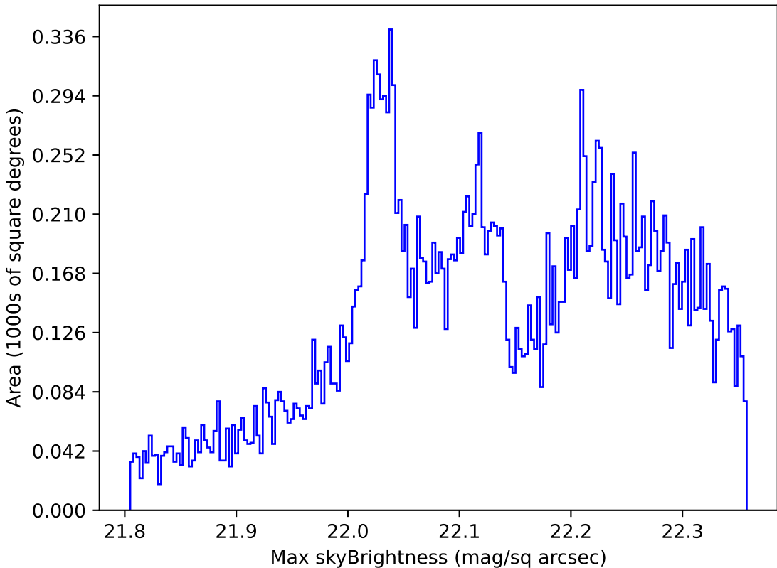
noroll_mjdp120_v3.4_10yrs All sky g band: Max skyBrightness
