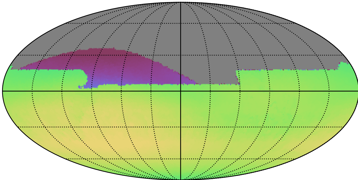
noroll_mjdp120_v3.4_10yrs All sky all bands: Max skyBrightness
