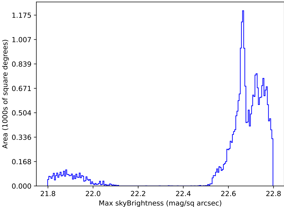
noroll_mjdp120_v3.4_10yrs All sky all bands: Max skyBrightness
