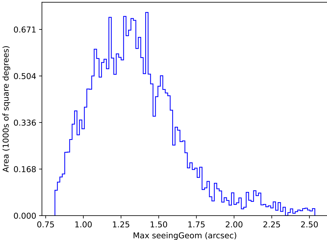
noroll_mjdp120_v3.4_10yrs Yr 1 z band: Max seeingGeom
