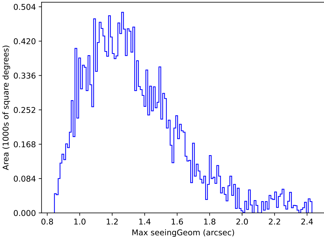
noroll_mjdp120_v3.4_10yrs Yr 1 y band: Max seeingGeom
