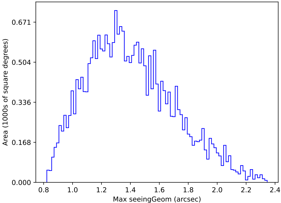
noroll_mjdp120_v3.4_10yrs Yr 1 r band: Max seeingGeom
