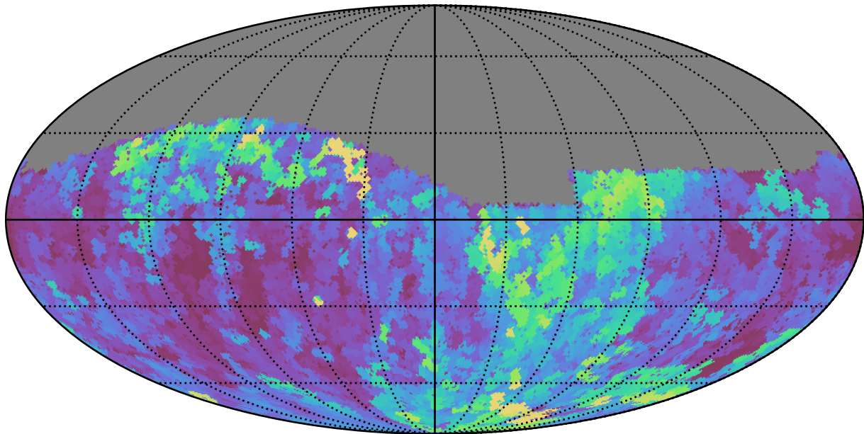
noroll_mjdp120_v3.4_10yrs Yr 1 g band: Max seeingGeom
