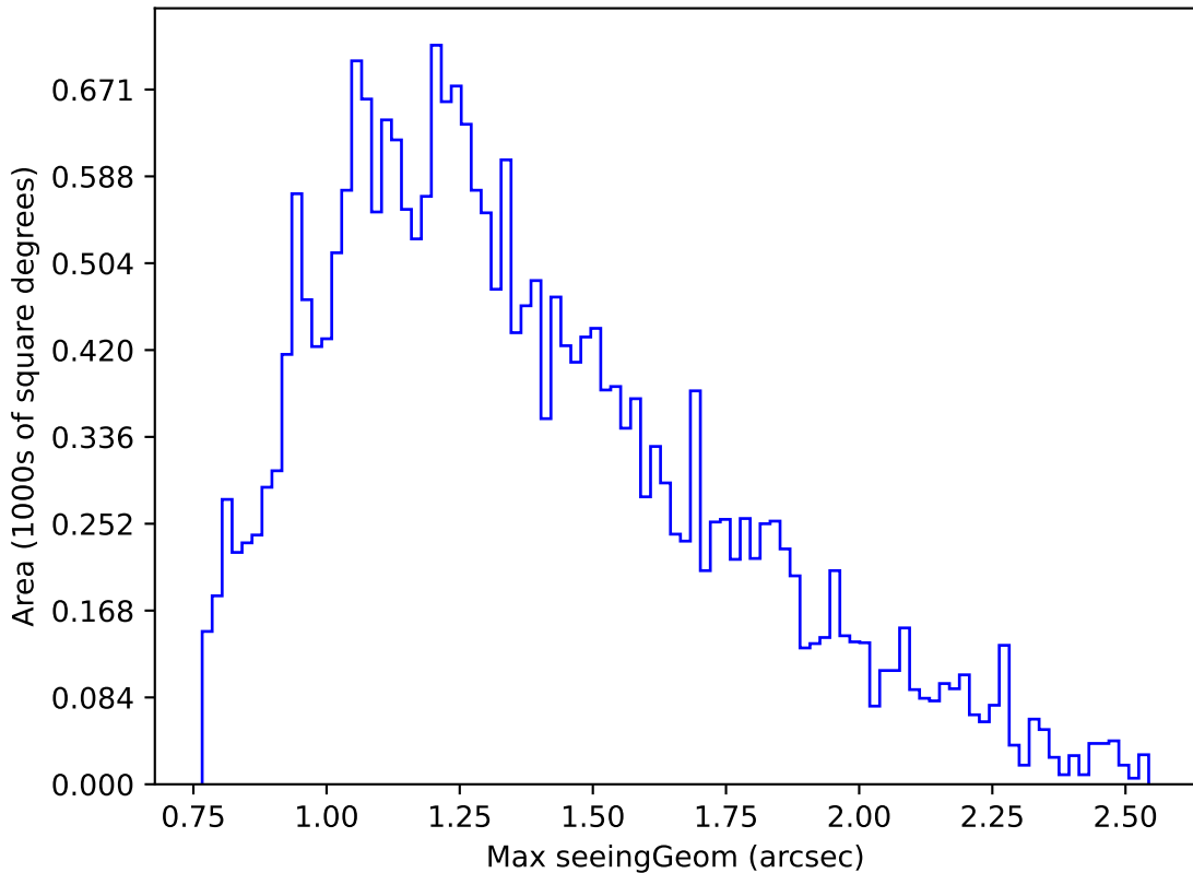
noroll_mjdp120_v3.4_10yrs Yr 1 g band: Max seeingGeom
