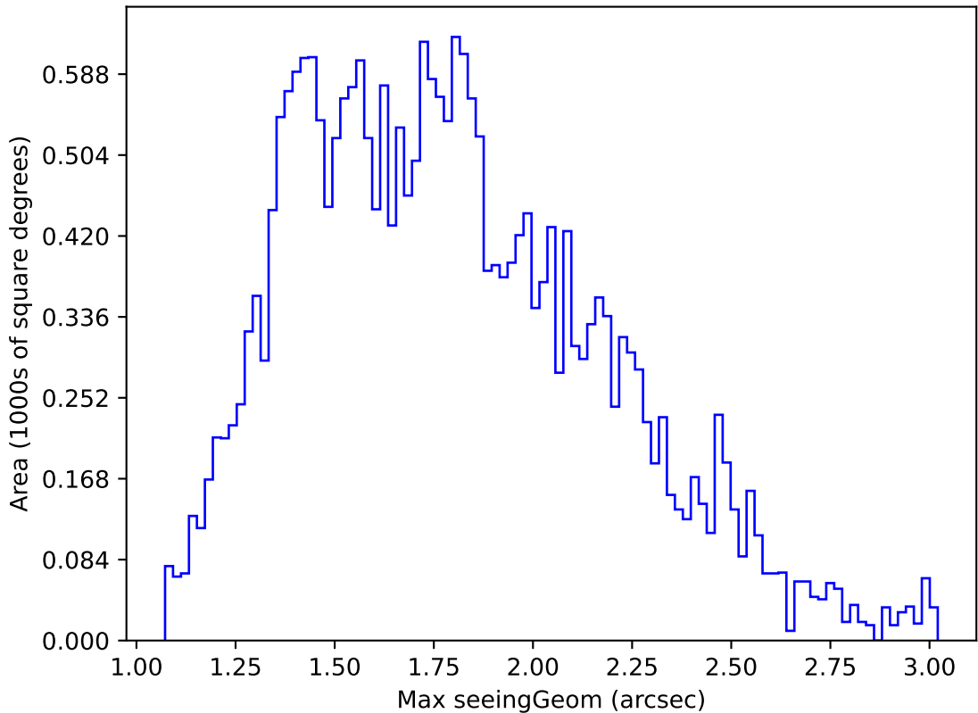
noroll_mjdp120_v3.4_10yrs Yr 1 all bands: Max seeingGeom
