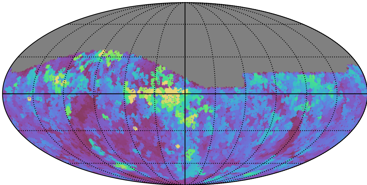
noroll_mjdp120_v3.4_10yrs Yr 1 z band: Max seeingEff
