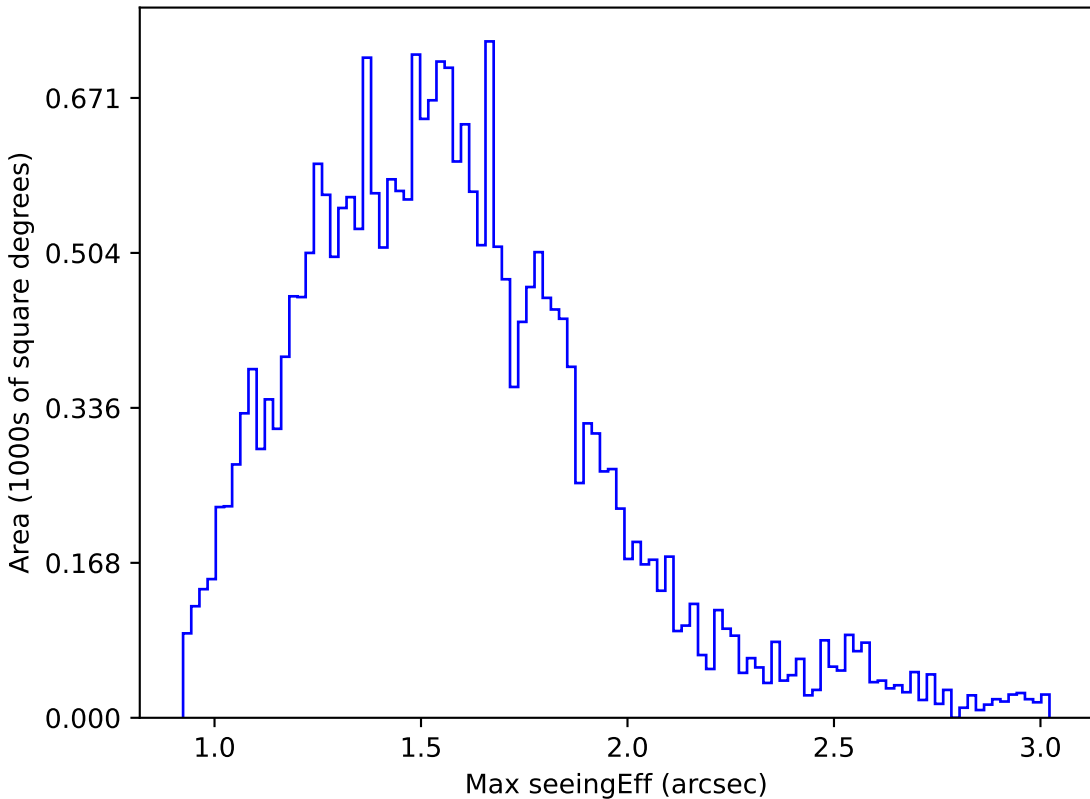
noroll_mjdp120_v3.4_10yrs Yr 1 z band: Max seeingEff
