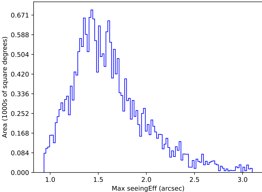
noroll_mjdp120_v3.4_10yrs Yr 1 u band: Max seeingEff
