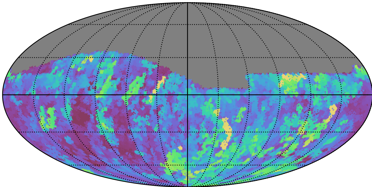
noroll_mjdp120_v3.4_10yrs Yr 1 r band: Max seeingEff
