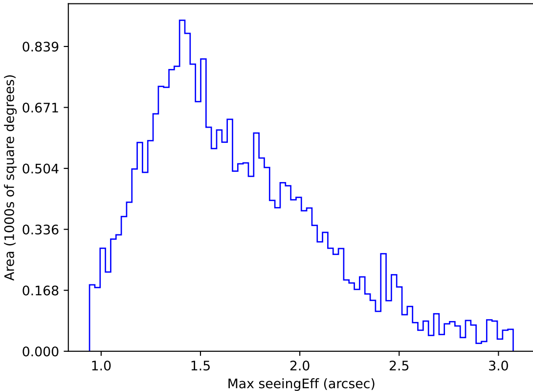
noroll_mjdp120_v3.4_10yrs Yr 1 i band: Max seeingEff
