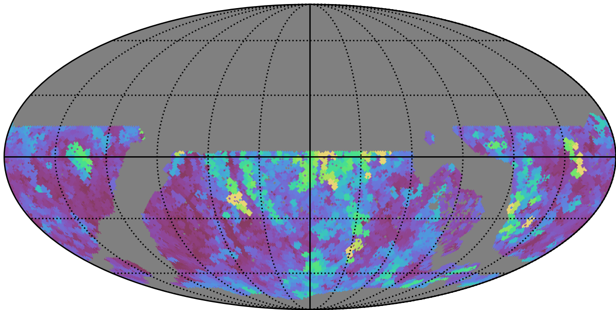
noroll_mjdp120_v3.4_10yrs WFD z band: Max seeingEff
