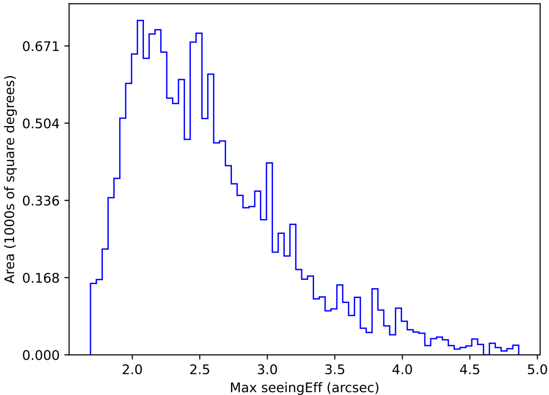
noroll_mjdp120_v3.4_10yrs WFD z band: Max seeingEff
