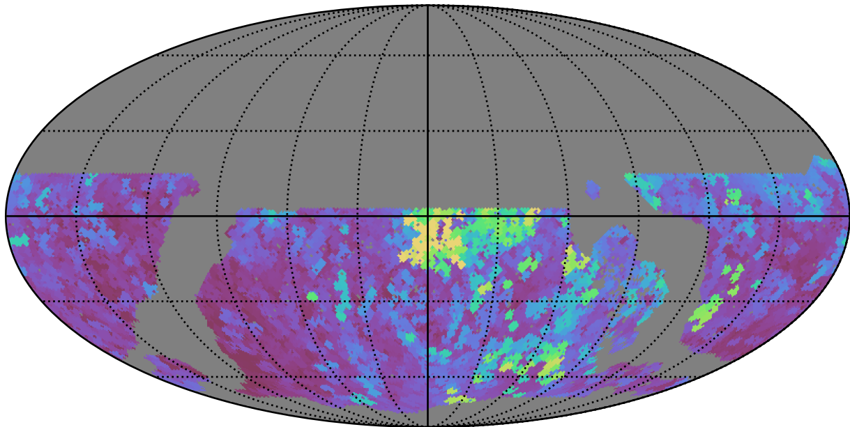
noroll_mjdp120_v3.4_10yrs WFD y band: Max seeingEff
