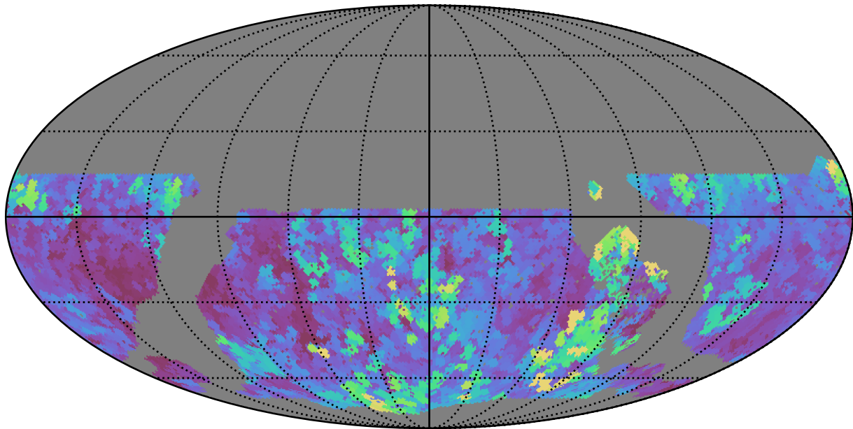
noroll_mjdp120_v3.4_10yrs WFD u band: Max seeingEff
