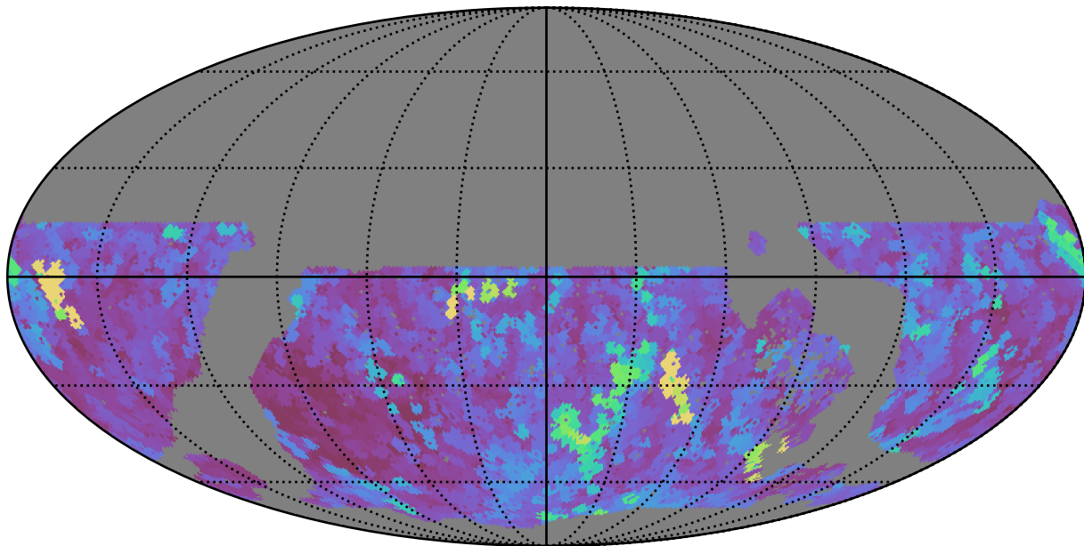
noroll_mjdp120_v3.4_10yrs WFD i band: Max seeingEff
