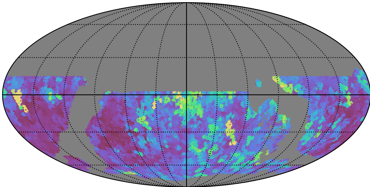
noroll_mjdp120_v3.4_10yrs WFD all bands: Max seeingEff
