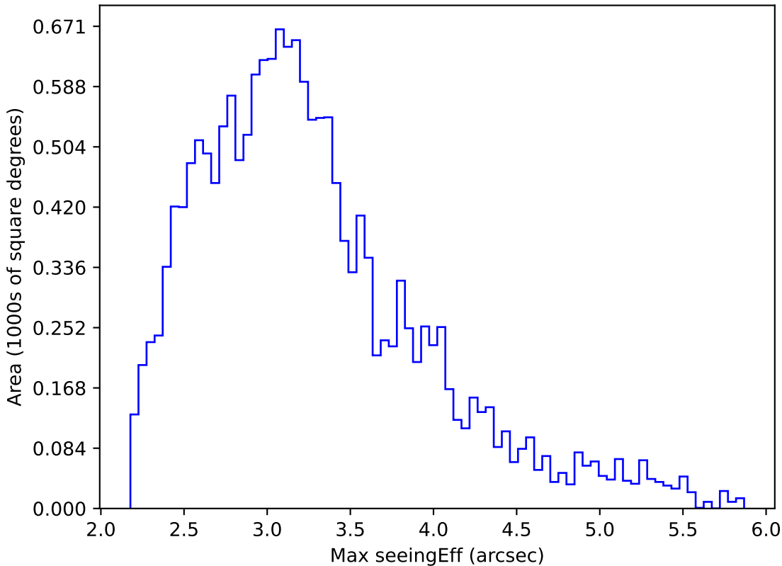
noroll_mjdp120_v3.4_10yrs WFD all bands: Max seeingEff
