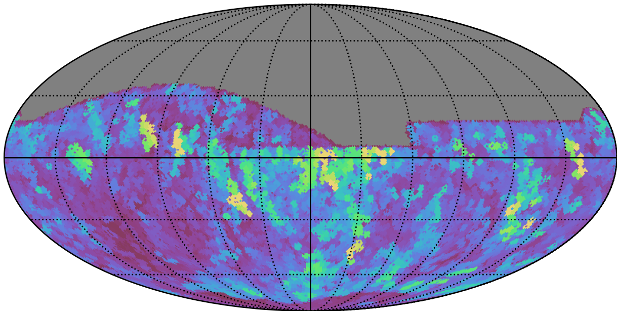
noroll_mjdp120_v3.4_10yrs All sky z band: Max seeingEff
