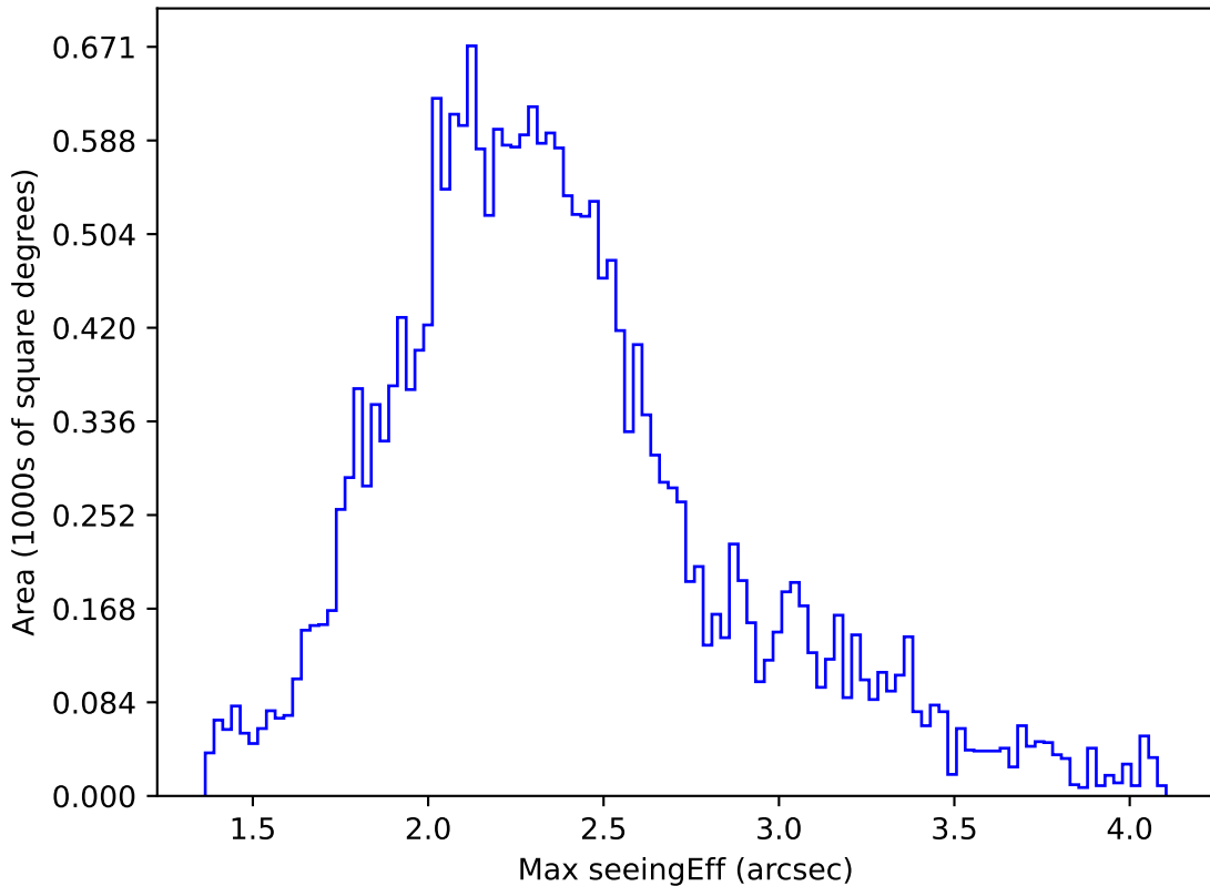
noroll_mjdp120_v3.4_10yrs All sky u band: Max seeingEff
