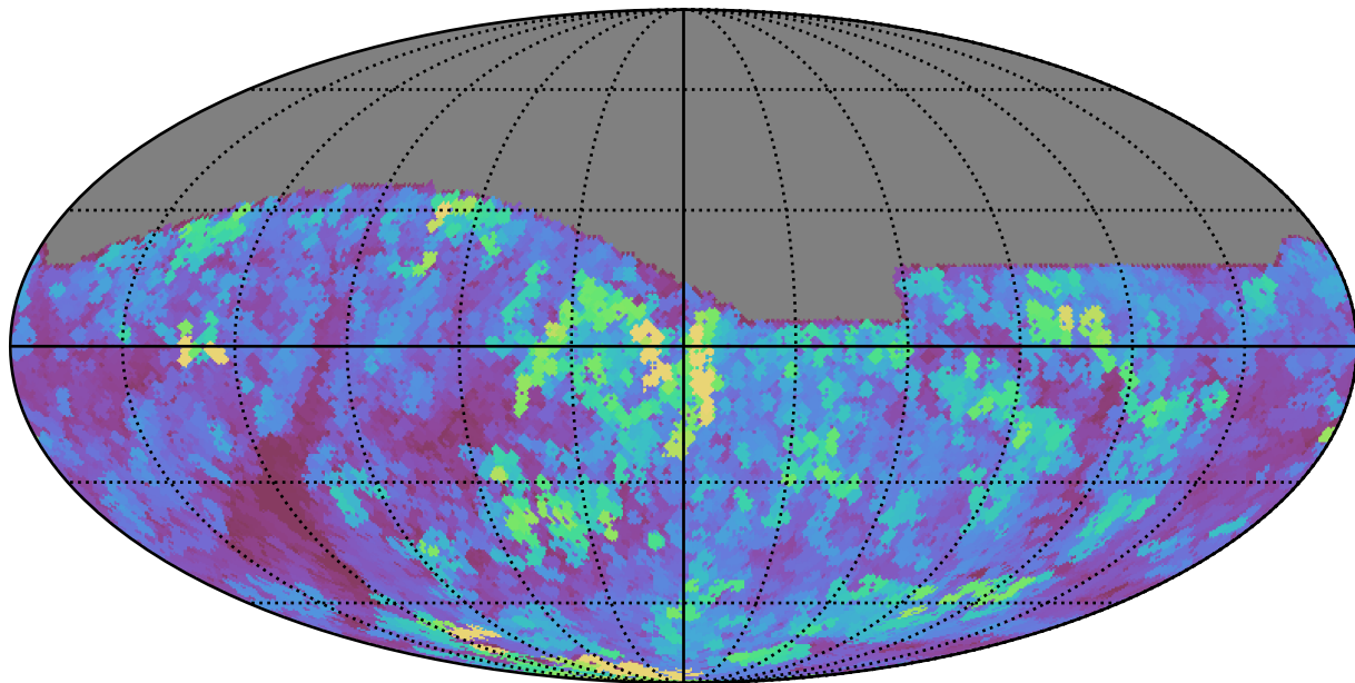
noroll_mjdp120_v3.4_10yrs All sky r band: Max seeingEff
