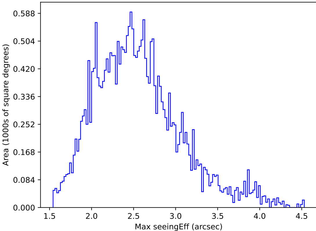
noroll_mjdp120_v3.4_10yrs All sky r band: Max seeingEff
