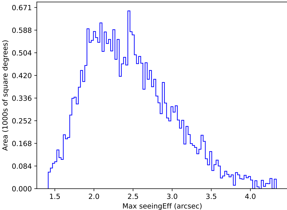
noroll_mjdp120_v3.4_10yrs All sky g band: Max seeingEff
