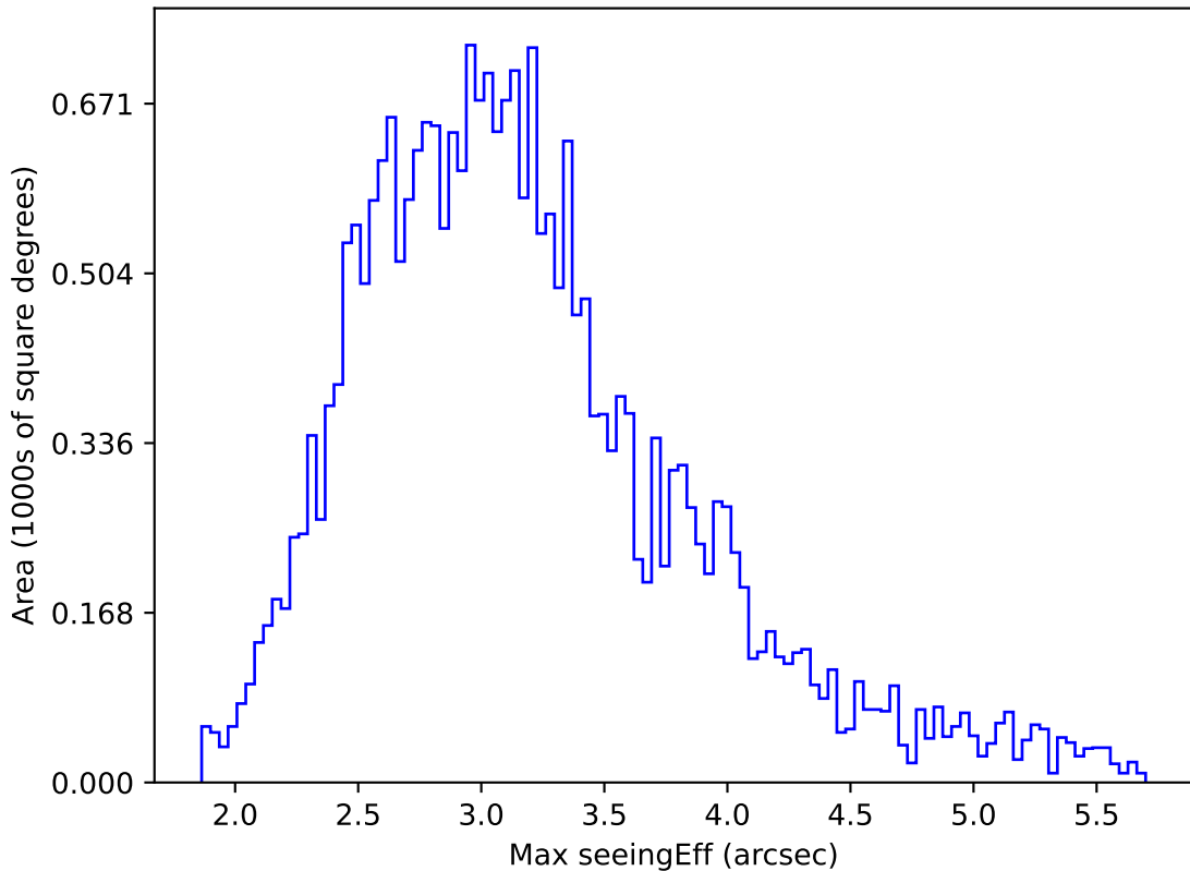
noroll_mjdp120_v3.4_10yrs All sky all bands: Max seeingEff
