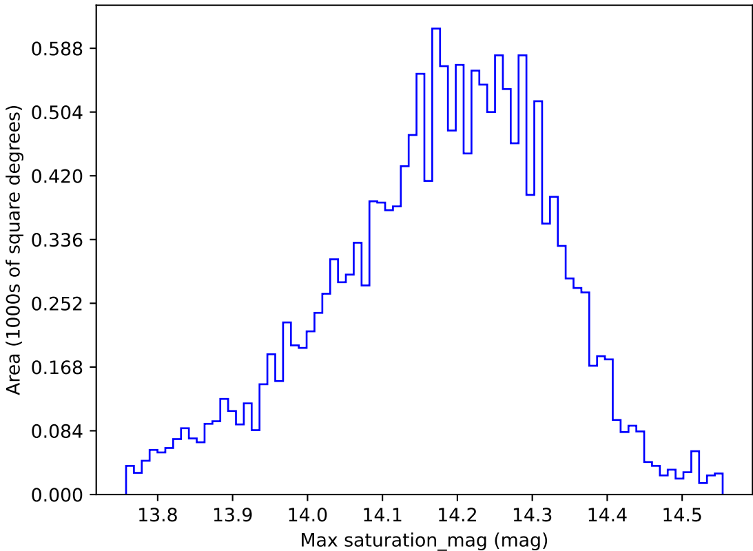
noroll_mjdp120_v3.4_10yrs WFD y band: Max saturation_mag
