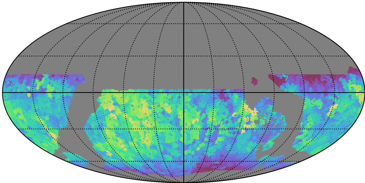
noroll_mjdp120_v3.4_10yrs WFD r band: Max saturation_mag
