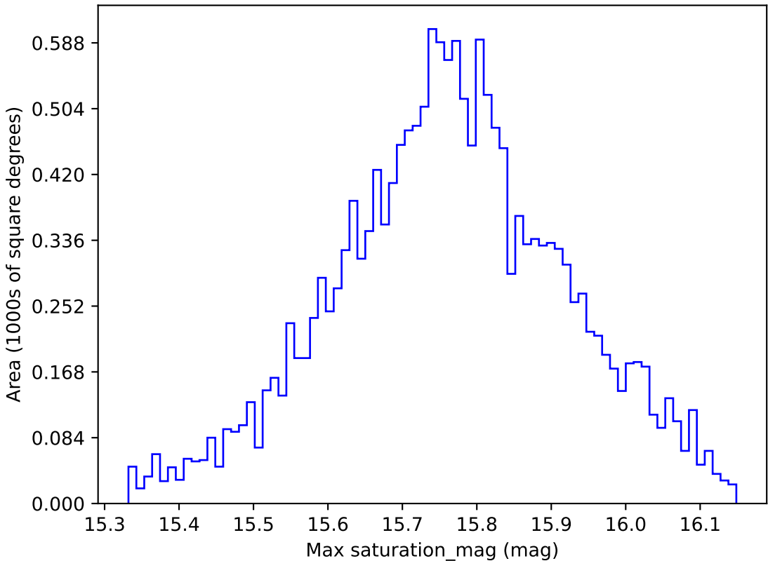
noroll_mjdp120_v3.4_10yrs WFD r band: Max saturation_mag
