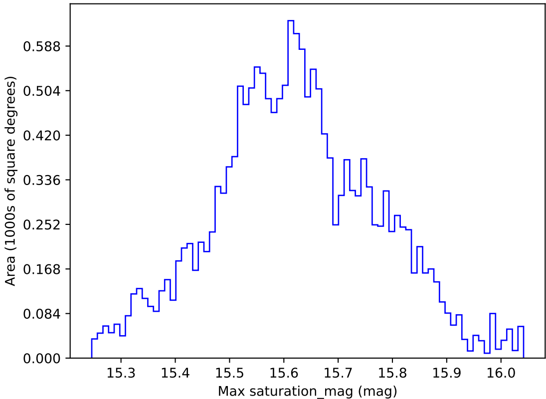
noroll_mjdp120_v3.4_10yrs WFD i band: Max saturation_mag
